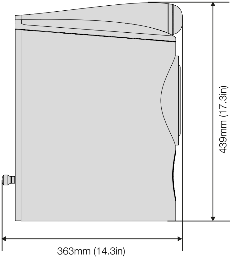
SIDE
