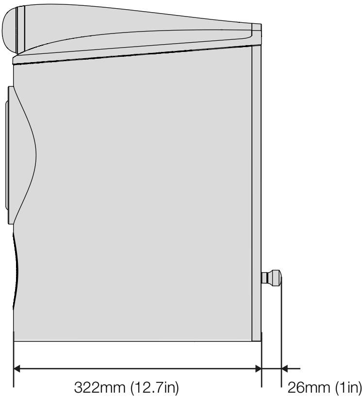
SIDE
