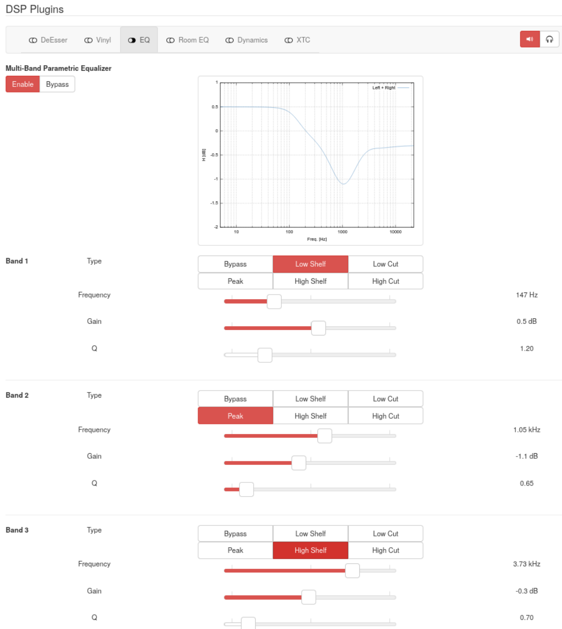
Figure 7: Equalizer plugin
