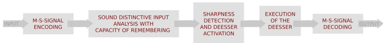
Figure 30: Block diagram of the Weiss De-Esser plugin
