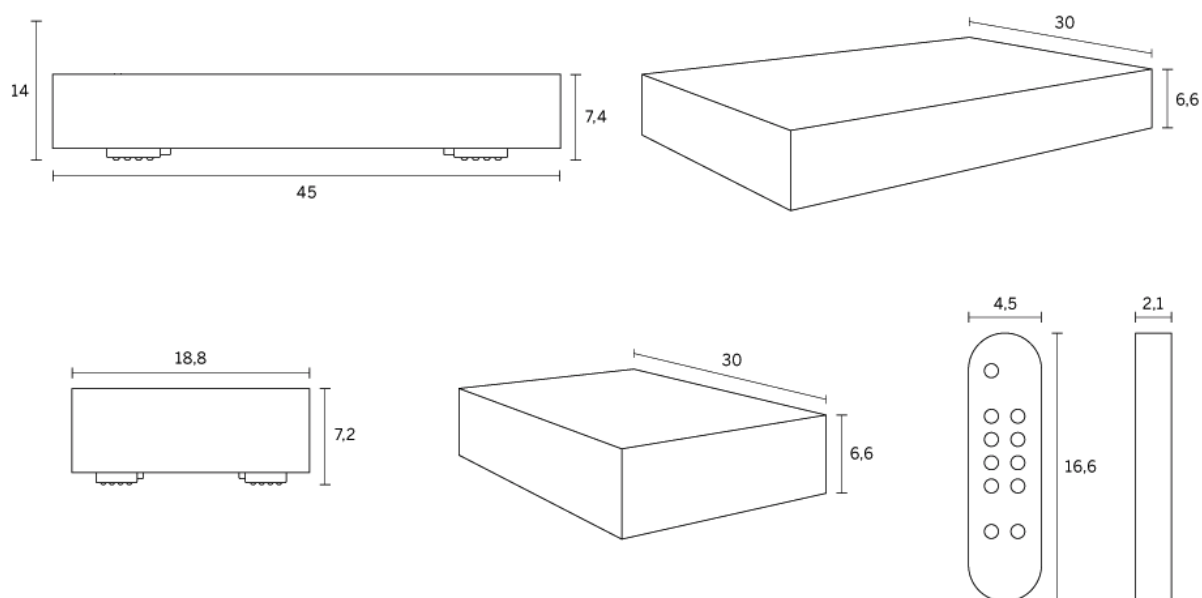
Figure 18: Engineering drawings of DAC501, DAC502 and IR remote control
