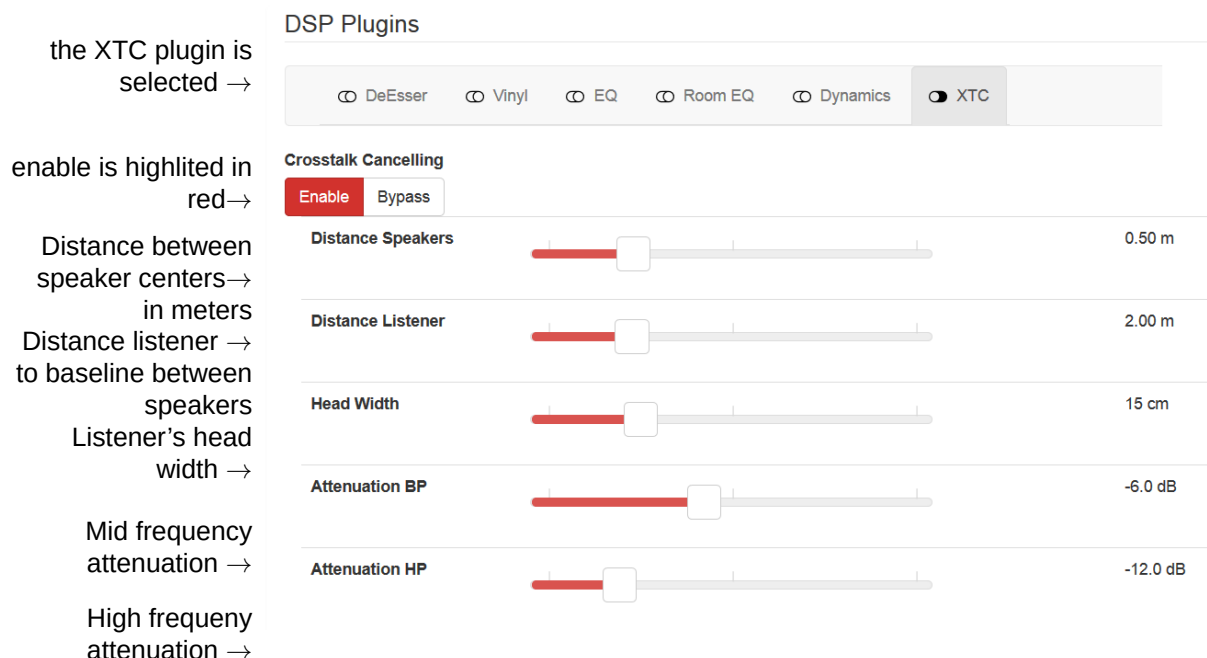
Figure 12: XTC plugin
